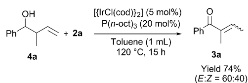
Scheme 4. Reaction of 4a with 2a .
