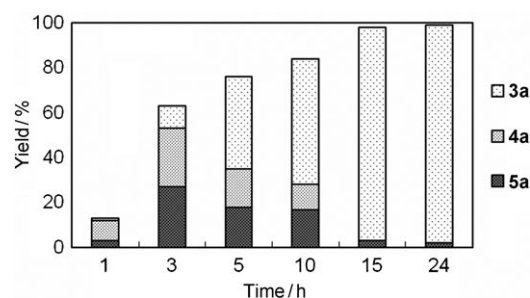
Figure 1. Time-course monitoring of the formation of 3a in the reaction of 1a with 2a under the conditions in Table 1, entry 1.
