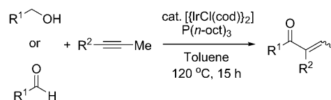
Scheme 1. Ir-catalyzed hydroacylation of 2-alkynes with primary alcohols or aldehydes.
