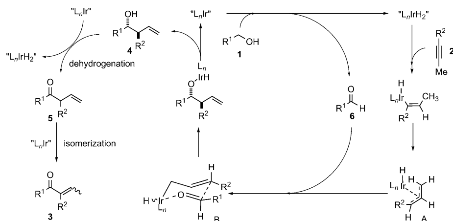
Scheme 5. A plausible reaction pathway for the formation of 3 via 4 and 5 as possible intermediates.
