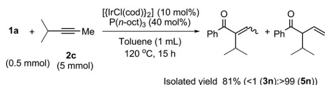
Scheme 2. Reaction of 1a with 2c .
