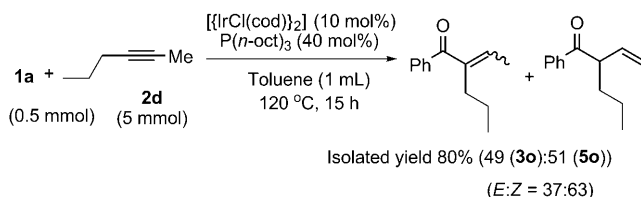
Scheme 3. Reaction of 1a with 2d .
